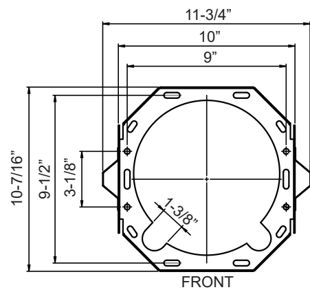
Ceiling Bracket
